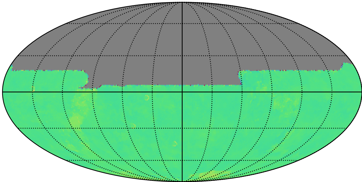
roll_uniform_eh_acc0.8_mjdp0_v3.4_10yrs y: Kuiper rotTelPos
