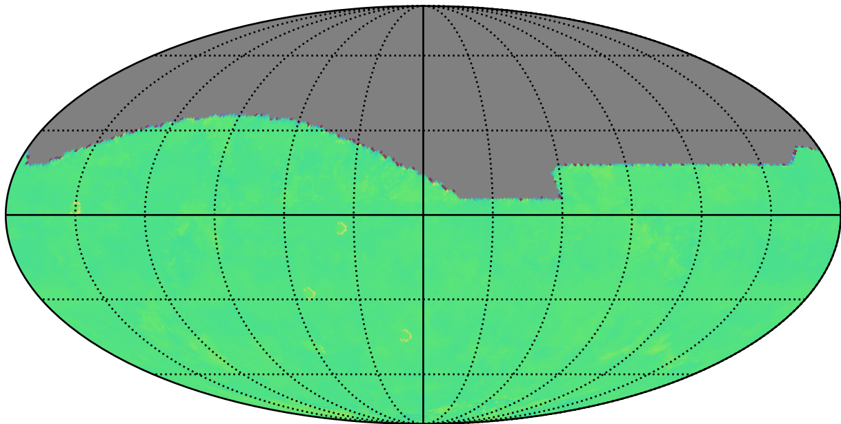
roll_uniform_eh_acc0.8_mjdp0_v3.4_10yrs r: Kuiper rotTelPos
