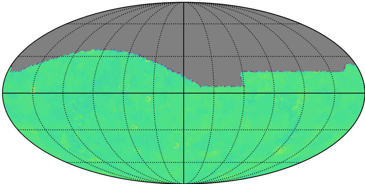
roll_uniform_eh_acc0.8_mjdp0_v3.4_10yrs g: Kuiper rotTelPos
