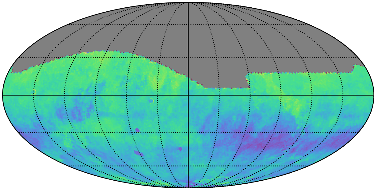
roll_uniform_eh_acc0.8_mjdp0_v3.4_10yrs r: Kuiper rotSkyPos
