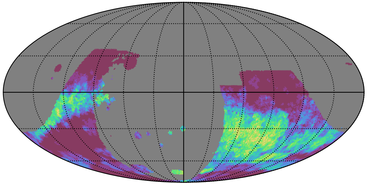
0.0 0.1 0.2 0.3 0.4 0.5 0.6 0.7 0.8 0.9 1.0 GalPlaneSeasonGapsTimescales_combined_map_Tau_25_0 (MJD mag)
