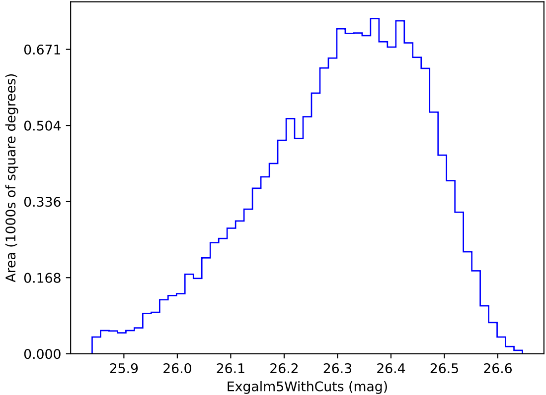
roll_uniform_eh_acc0.8_mjdp0_v3.4_10yrs i band non-DD year 9: ExgalM5WithCuts
