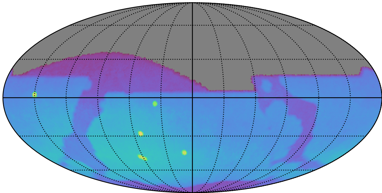
roll_uniform_eh_acc0.8_mjdp0_v3.4_10yrs : Brown Dwarf, L7
