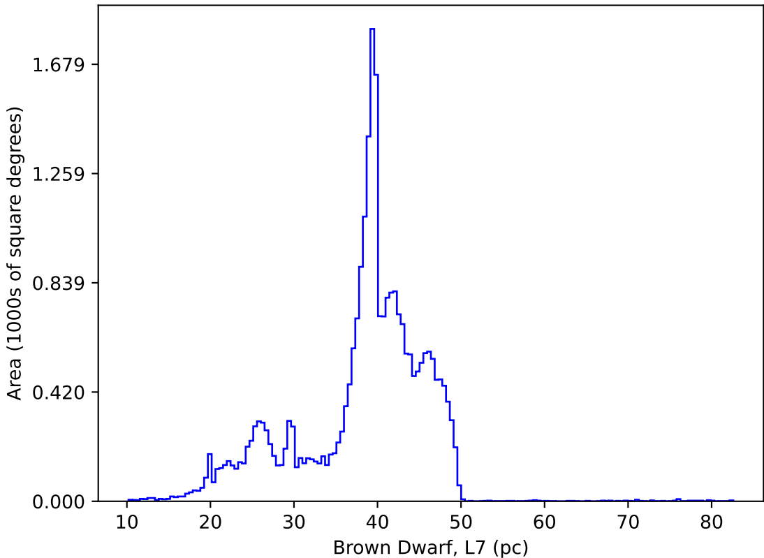
roll_uniform_eh_acc0.8_mjdp0_v3.4_10yrs : Brown Dwarf, L7
