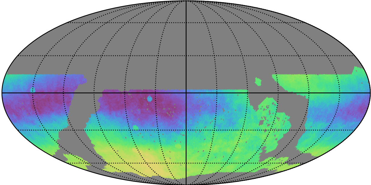
roll_uniform_eh_acc0.8_mjdp0_v3.4_10yrs WFD: Parallax-DCR degeneracy @ 24.0
