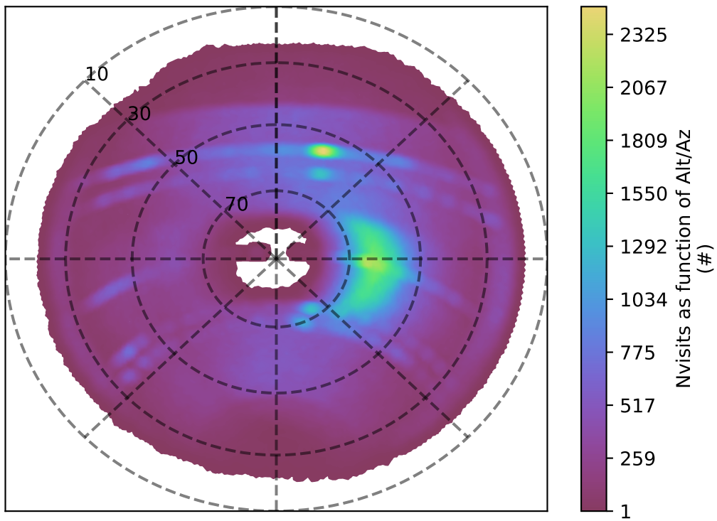
roll_uniform_eh_acc0.8_mjdp0_v3.4_10yrs z band: Nvisits as function of Alt/Az
