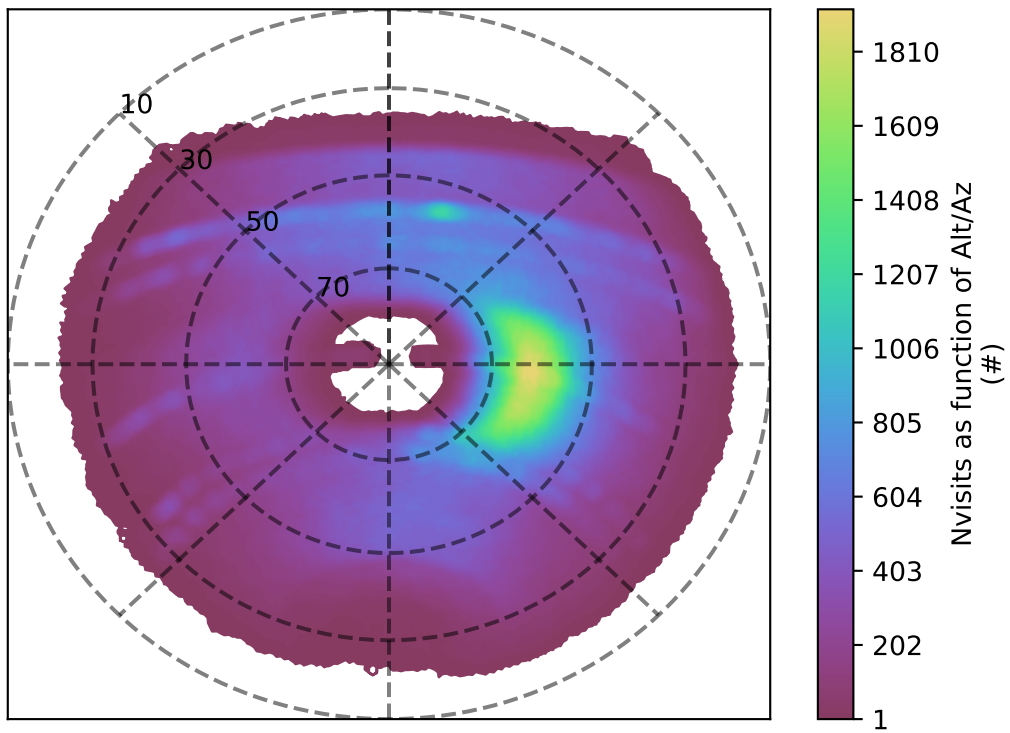
roll_uniform_eh_acc0.8_mjdp0_v3.4_10yrs y band: Nvisits as function of Alt/Az
