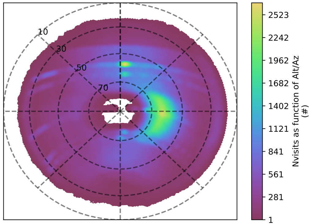
roll_uniform_eh_acc0.8_mjdp0_v3.4_10yrs i band: Nvisits as function of Alt/Az
