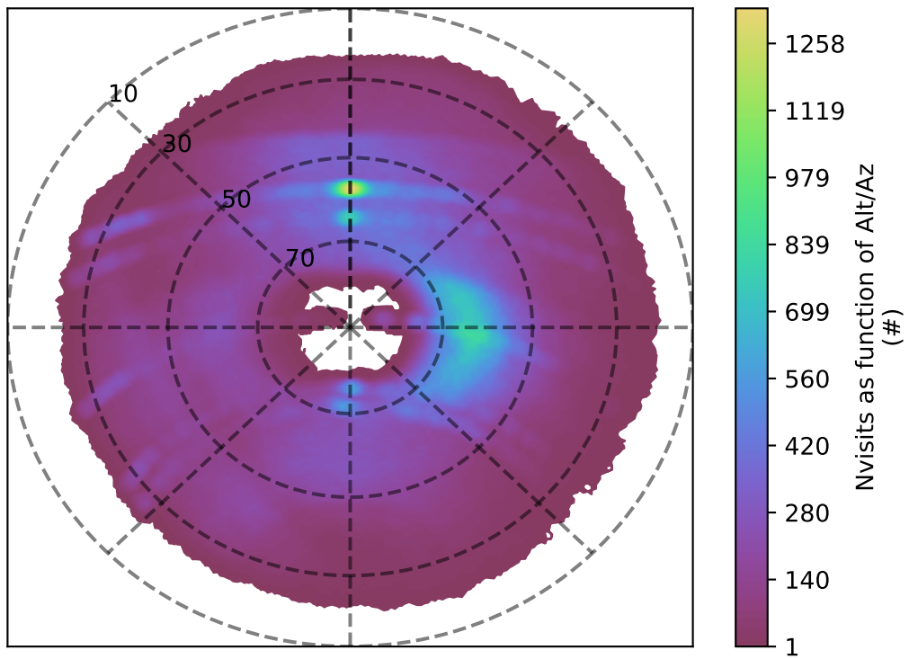
roll_uniform_eh_acc0.8_mjdp0_v3.4_10yrs g band: Nvisits as function of Alt/Az
