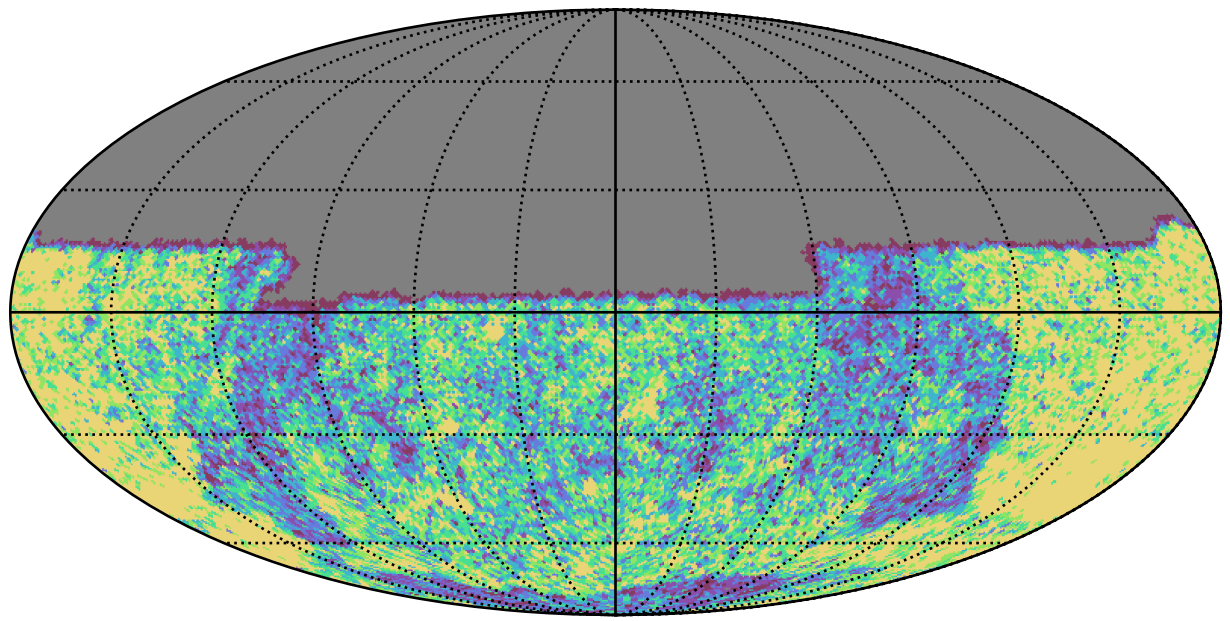
roll_uniform_eh_acc0.8_mjdp0_v3.4_10yrs Yr 1 u band: NVisits
