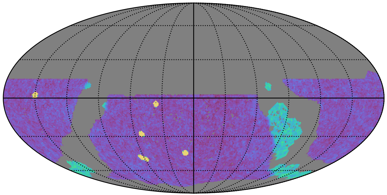
roll_uniform_eh_acc0.8_mjdp0_v3.4_10yrs WFD g band: NVisits
