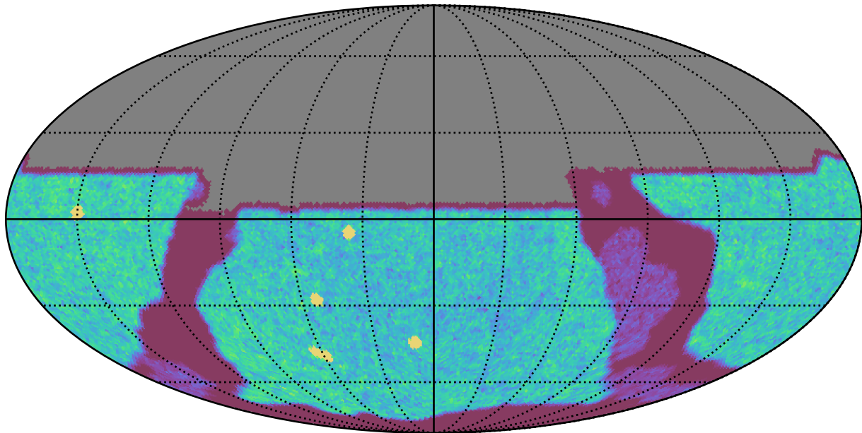
roll_uniform_eh_acc0.8_mjdp0_v3.4_10yrs All sky u band: NVisits
