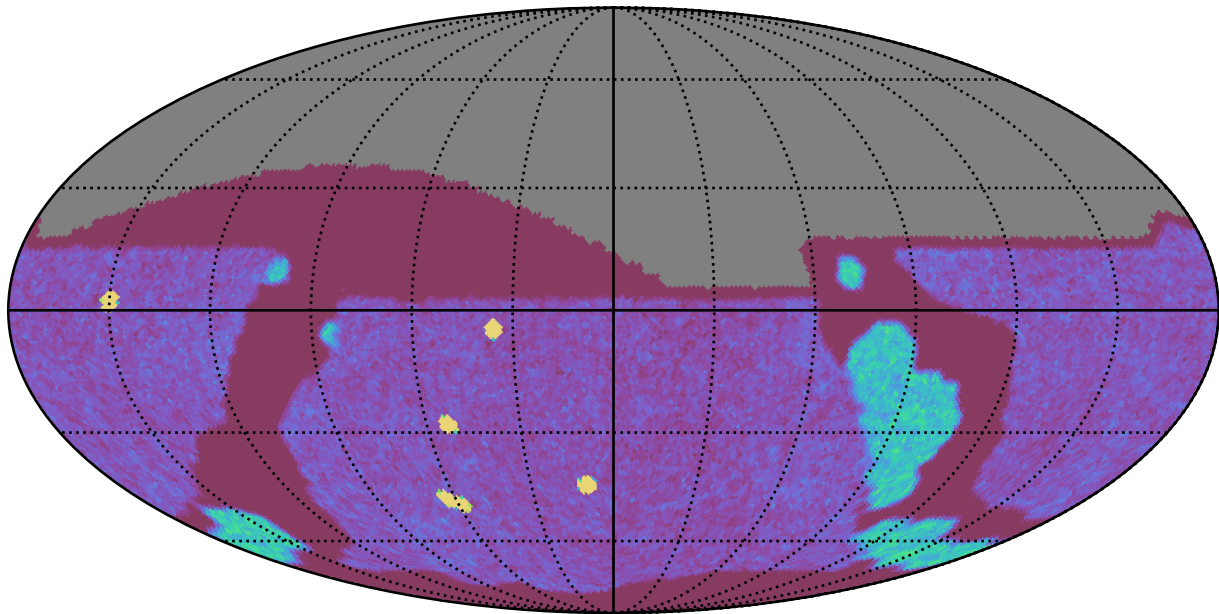
roll_uniform_eh_acc0.8_mjdp0_v3.4_10yrs All sky g band: NVisits
