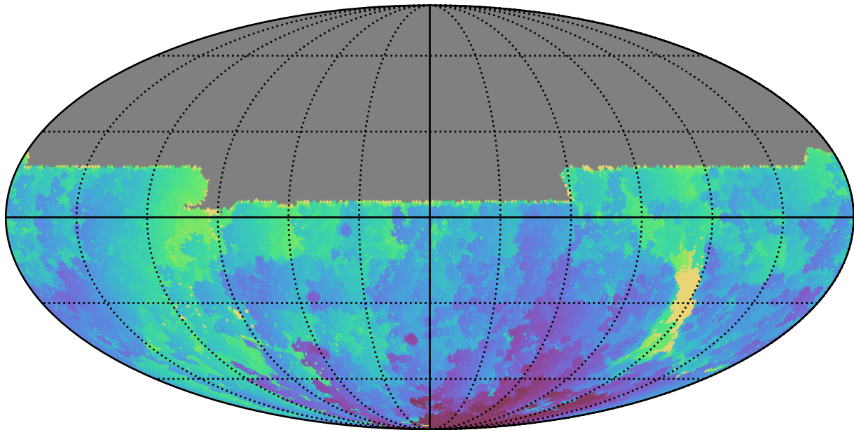
roll_uniform_eh_acc0.8_mjdp0_v3.4_10yrs All sky u band: Min HA
