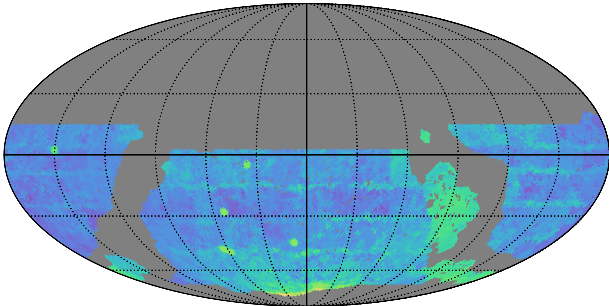
roll_uniform_eh_acc0.8_mjdp0_v3.4_10yrs WFD r band: Median Season Length
