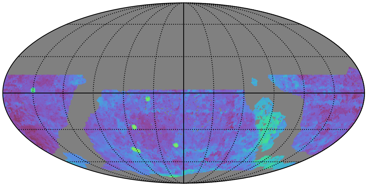
roll_uniform_eh_acc0.8_mjdp0_v3.4_10yrs WFD g band: Median Season Length
