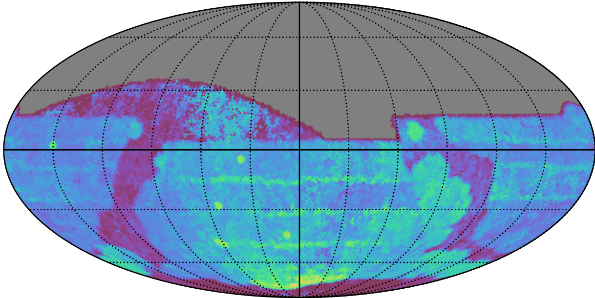
roll_uniform_eh_acc0.8_mjdp0_v3.4_10yrs All sky z band: Median Season Length
