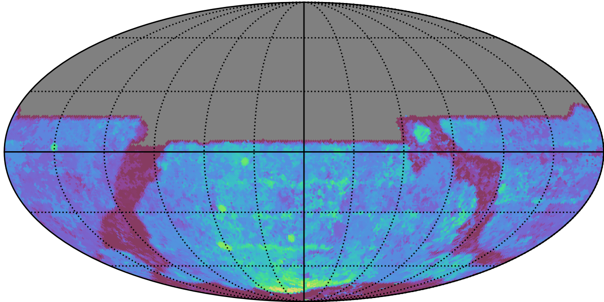
roll_uniform_eh_acc0.8_mjdp0_v3.4_10yrs All sky y band: Median Season Length
