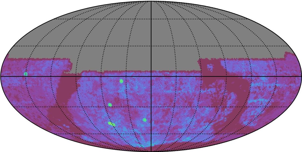
roll_uniform_eh_acc0.8_mjdp0_v3.4_10yrs All sky u band: Median Season Length
