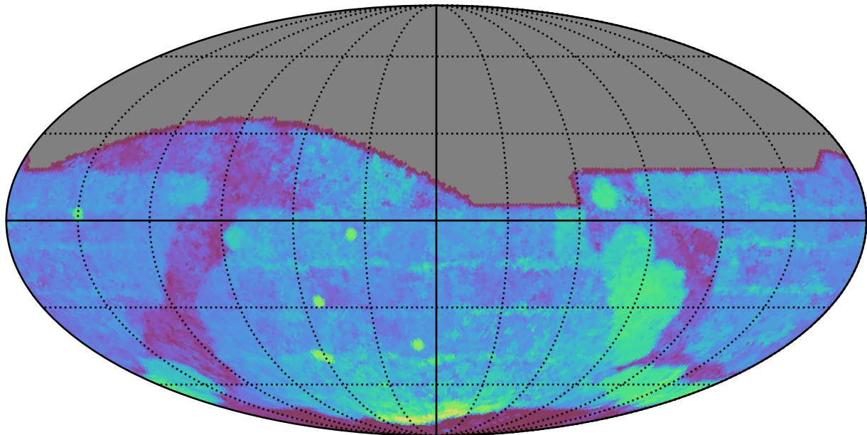
roll_uniform_eh_acc0.8_mjdp0_v3.4_10yrs All sky r band: Median Season Length
