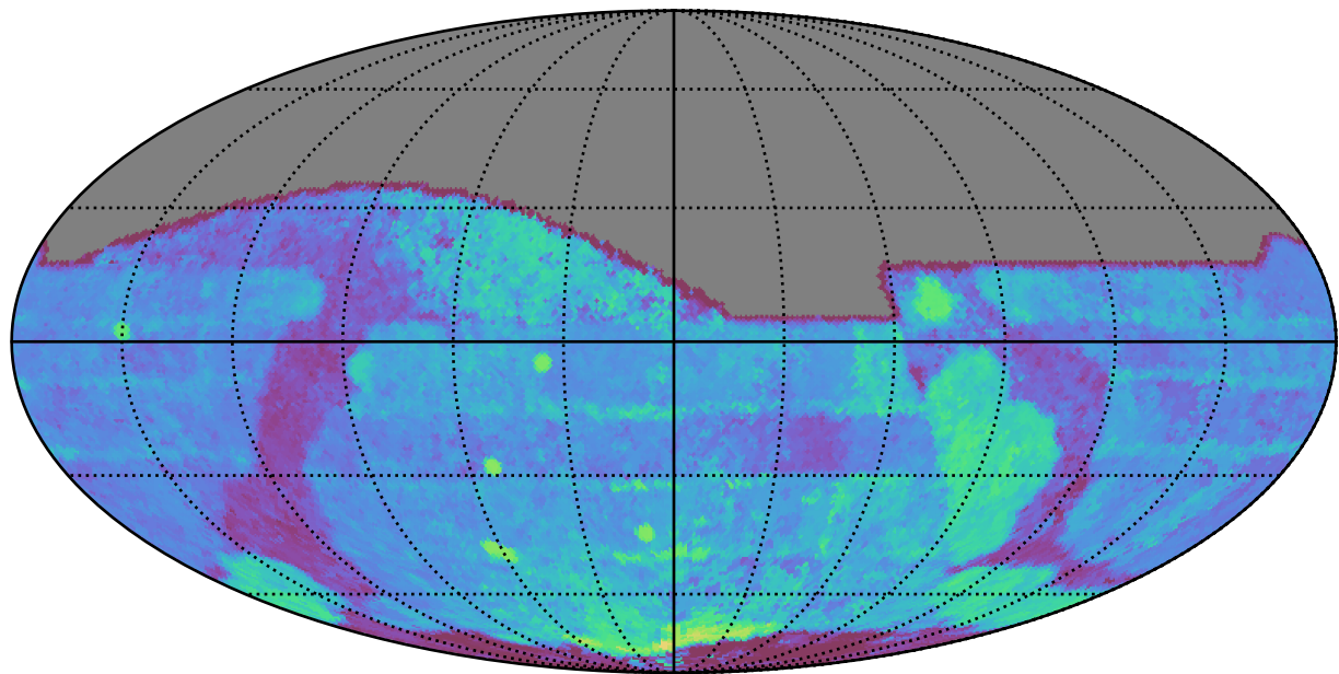
roll_uniform_eh_acc0.8_mjdp0_v3.4_10yrs All sky i band: Median Season Length
