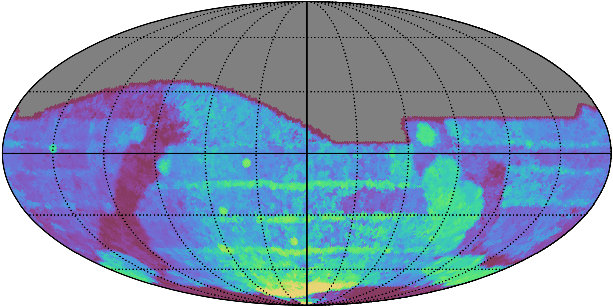
roll_uniform_eh_acc0.8_mjdp0_v3.4_10yrs All sky all bands: Median Season Length
