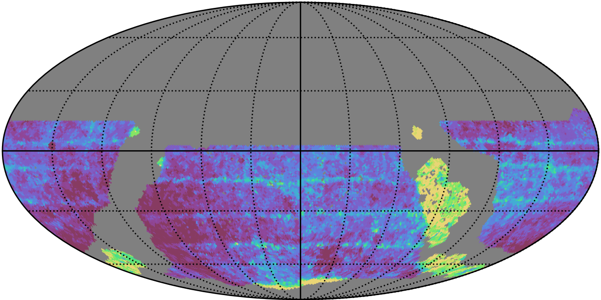
roll_uniform_eh_acc0.8_mjdp0_v3.4_10yrs WFD z band: Median Inter-Night Gap
