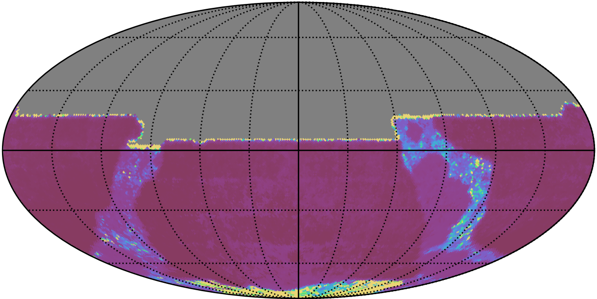
roll_uniform_eh_acc0.8_mjdp0_v3.4_10yrs All sky y band: Median Inter-Night Gap
