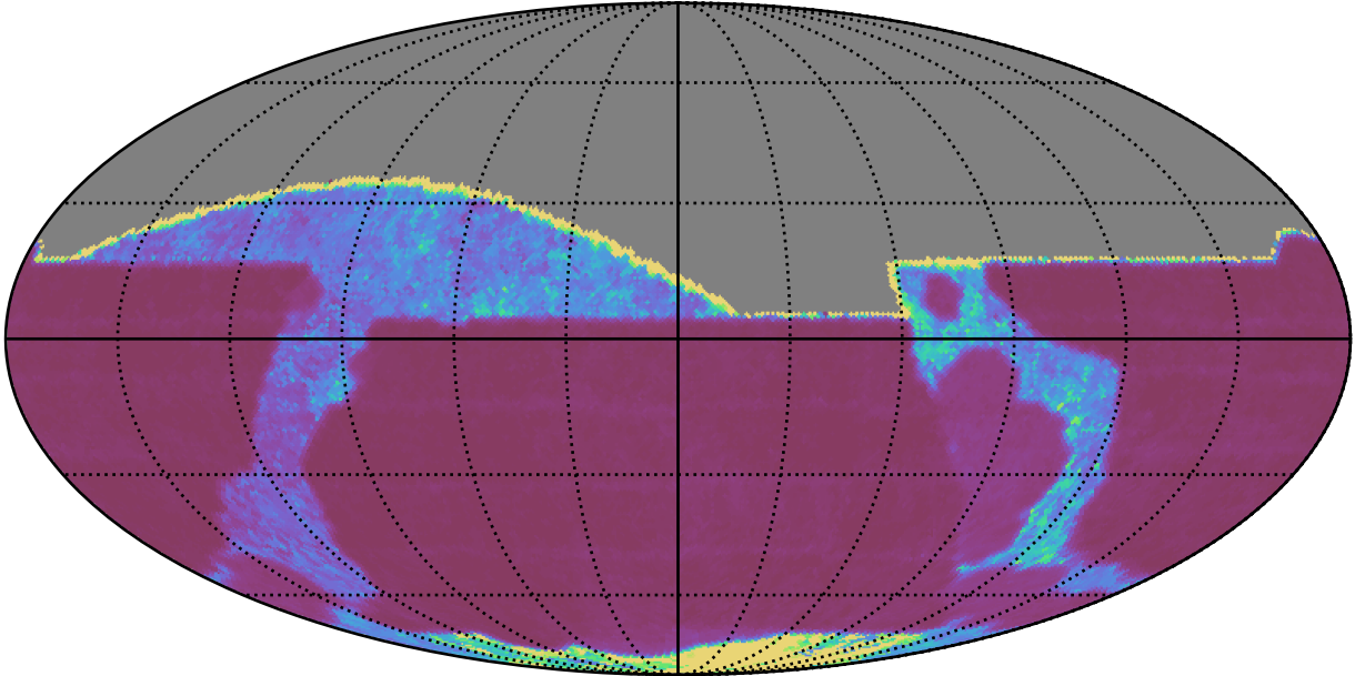
roll_uniform_eh_acc0.8_mjdp0_v3.4_10yrs All sky i band: Median Inter-Night Gap
