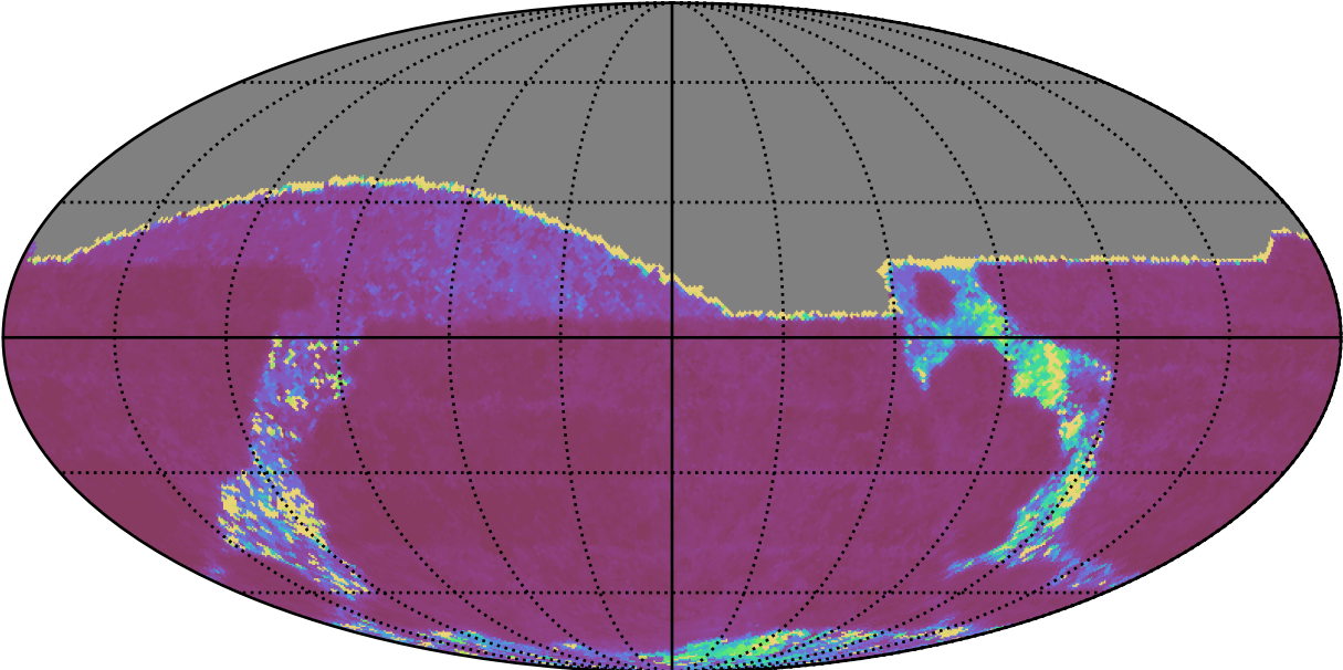
roll_uniform_eh_acc0.8_mjdp0_v3.4_10yrs All sky g band: Median Inter-Night Gap
