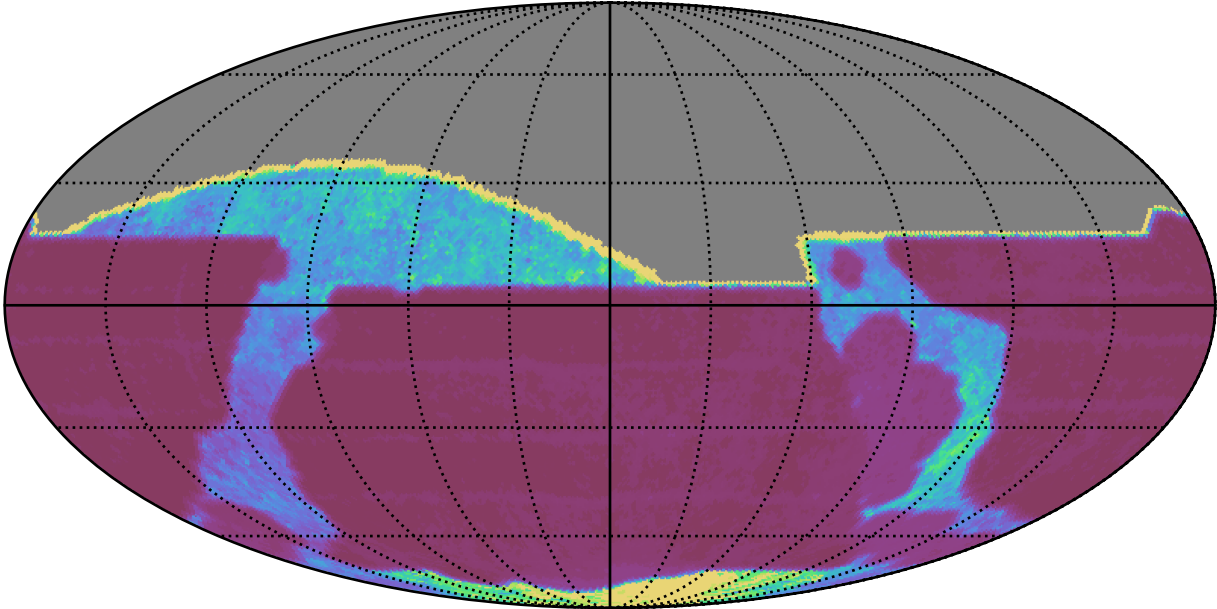
roll_uniform_eh_acc0.8_mjdp0_v3.4_10yrs All sky all bands: Median Inter-Night Gap
