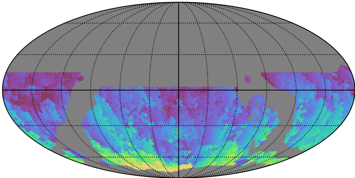
roll_uniform_eh_acc0.8_mjdp0_v3.4_10yrs WFD g band: Max HA
