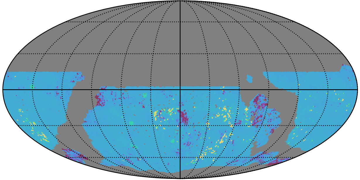
roll_uniform_eh_acc0.8_mjdp0_v3.4_10yrs WFD ug bands: 75th Percentile Intranight Timespan
