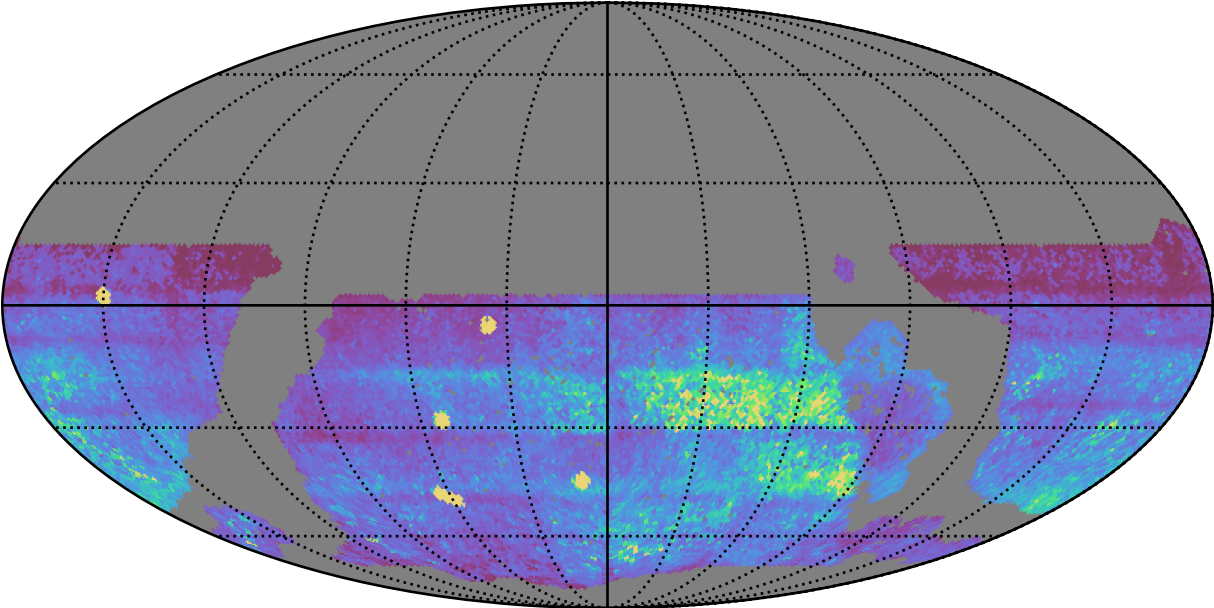
roll_uniform_eh_acc0.8_mjdp0_v3.4_10yrs WFD: 75th Percentile Intranight Timespan
