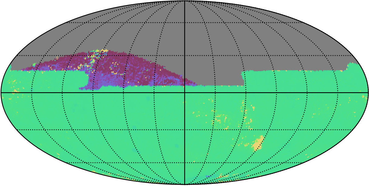
roll_uniform_eh_acc0.8_mjdp0_v3.4_10yrs All sky zy bands: 75th Percentile Intranight Timespan
