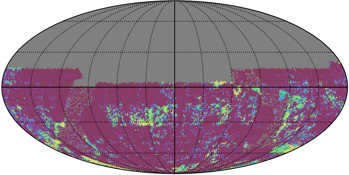
roll_uniform_eh_acc0.8_mjdp0_v3.4_10yrs All sky u band: 75th Percentile Intranight Timespan
