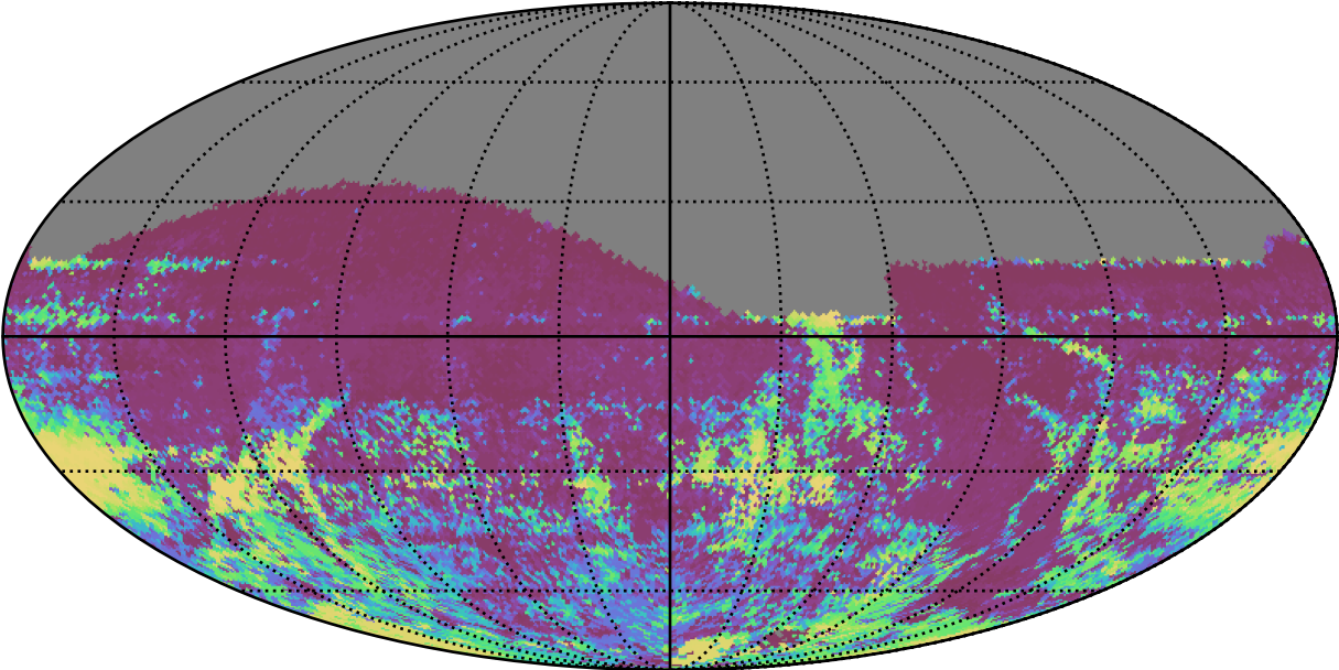
roll_uniform_eh_acc0.8_mjdp0_v3.4_10yrs All sky r band: 75th Percentile Intranight Timespan
