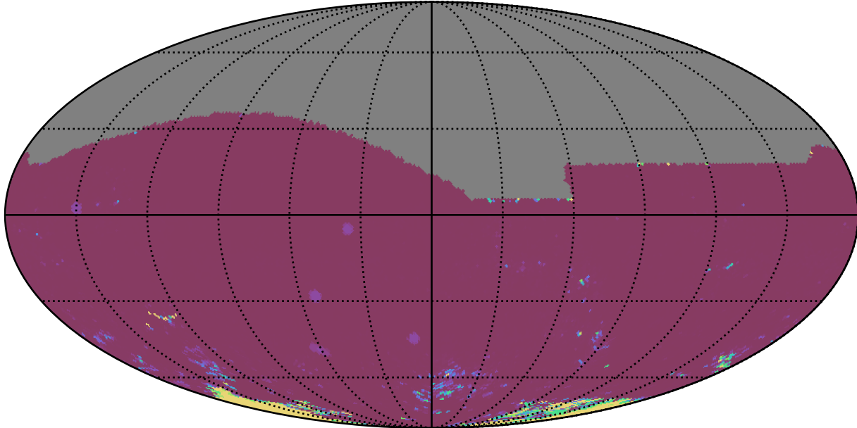
roll_uniform_eh_acc0.8_mjdp0_v3.4_10yrs All sky iz bands: 75th Percentile Intranight Timespan
