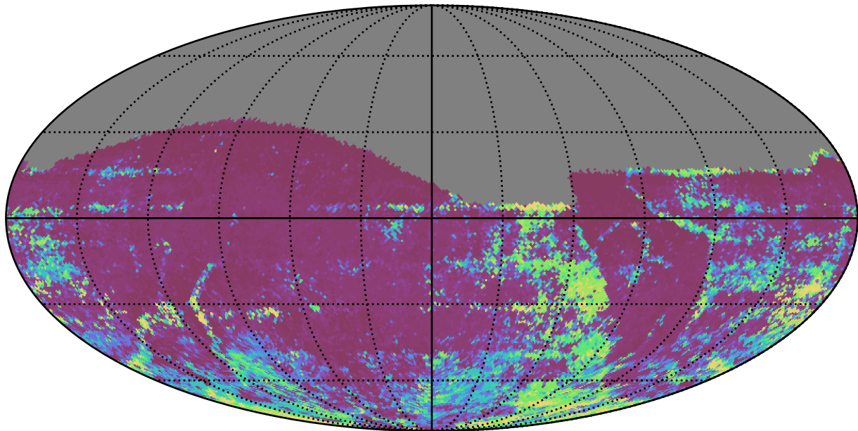
roll_uniform_eh_acc0.8_mjdp0_v3.4_10yrs All sky i band: 75th Percentile Intranight Timespan
