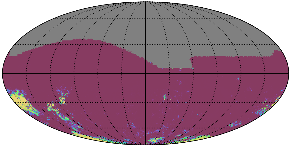
roll_uniform_eh_acc0.8_mjdp0_v3.4_10yrs All sky gr bands: 75th Percentile Intranight Timespan
