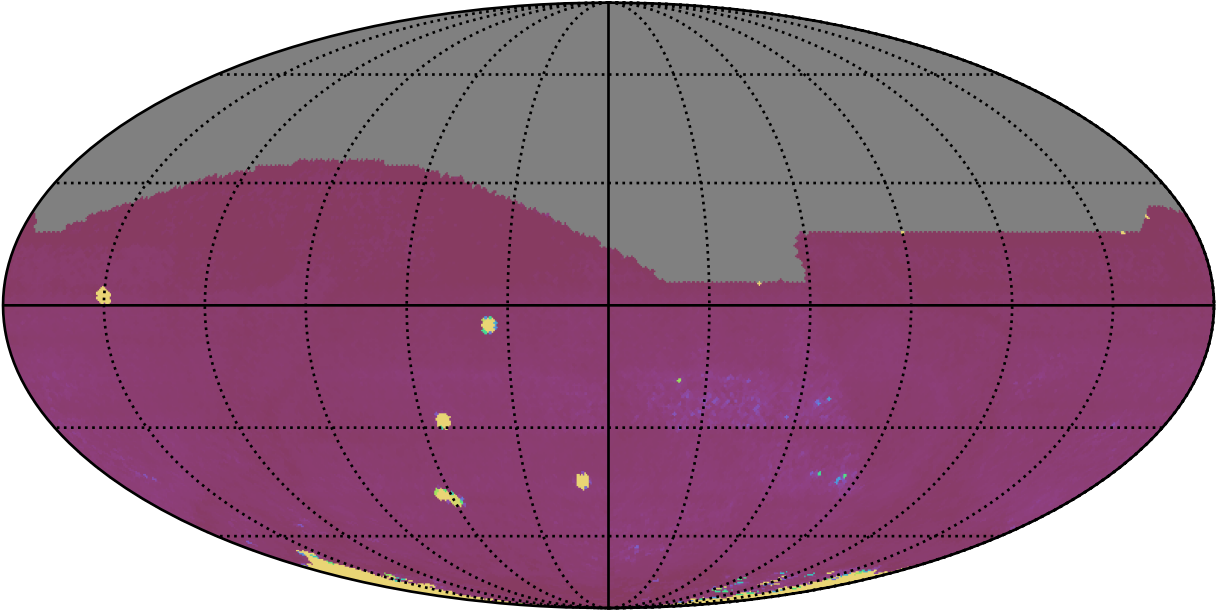
roll_uniform_eh_acc0.8_mjdp0_v3.4_10yrs All sky all bands: 75th Percentile Intranight Timespan
