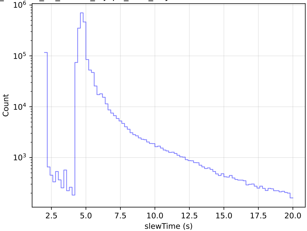
roll_uniform_eh_acc0.8_mjdp0_v3.4_10yrs All visits: Zoom Slew Time Histogram
