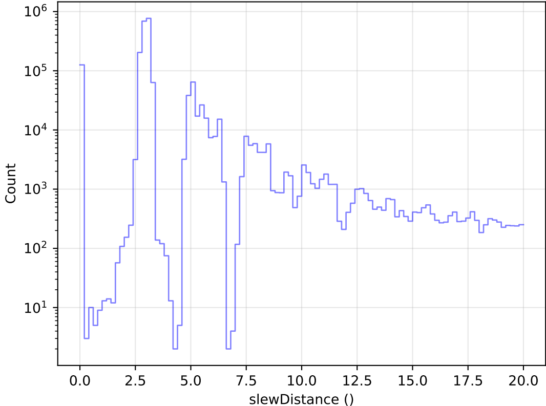
roll_uniform_eh_acc0.8_mjdp0_v3.4_10yrs All visits: Zoom Slew Distance Histogram
