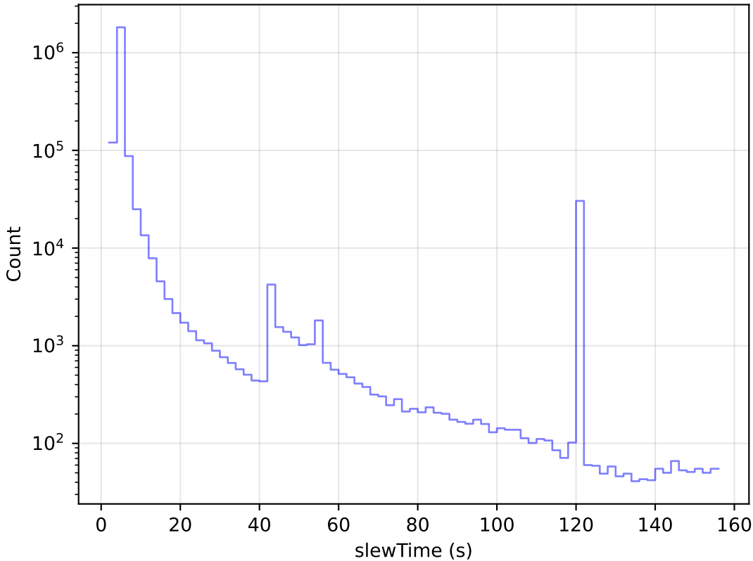
roll_uniform_eh_acc0.8_mjdp0_v3.4_10yrs All visits: Slew Time Histogram
