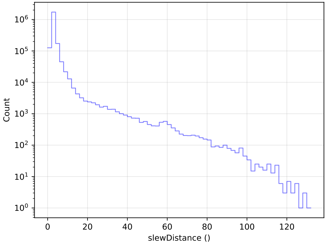
roll_uniform_eh_acc0.8_mjdp0_v3.4_10yrs All visits: Slew Distance Histogram
