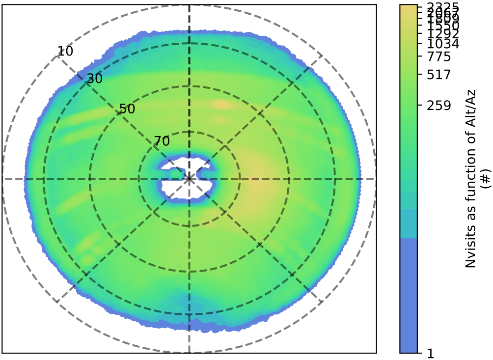
roll_uniform_eh_acc0.8_mjdp0_v3.4_10yrs z: Nvisits as function of Alt/Az
