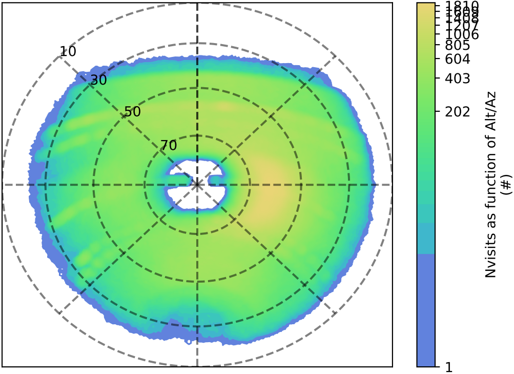
roll_uniform_eh_acc0.8_mjdp0_v3.4_10yrs y: Nvisits as function of Alt/Az
