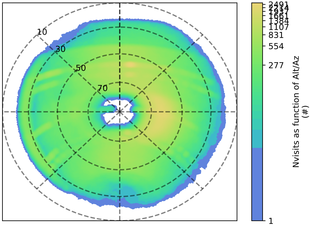
roll_uniform_eh_acc0.8_mjdp0_v3.4_10yrs r: Nvisits as function of Alt/Az
