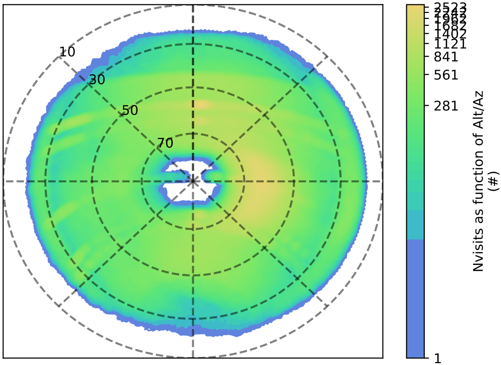
roll_uniform_eh_acc0.8_mjdp0_v3.4_10yrs i: Nvisits as function of Alt/Az
