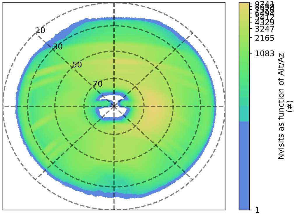
roll_uniform_eh_acc0.8_mjdp0_v3.4_10yrs : Nvisits as function of Alt/Az
